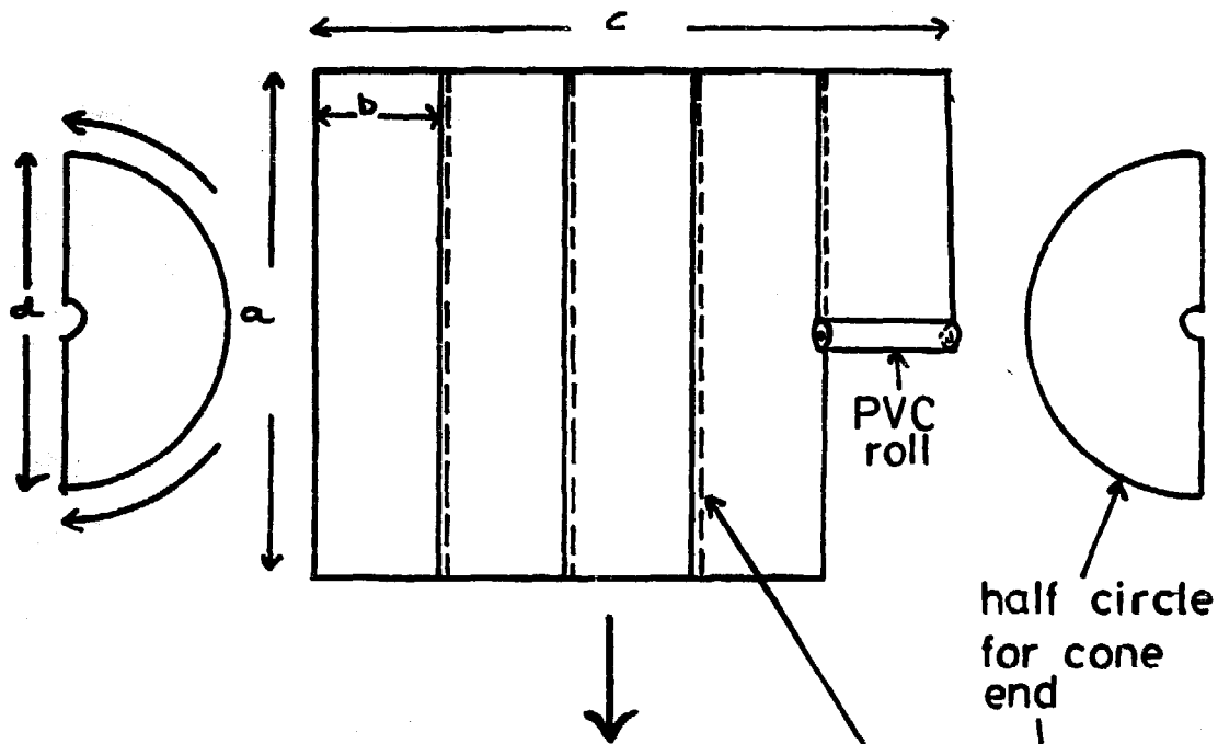
Fig 2 Construction of tube biogas digester
