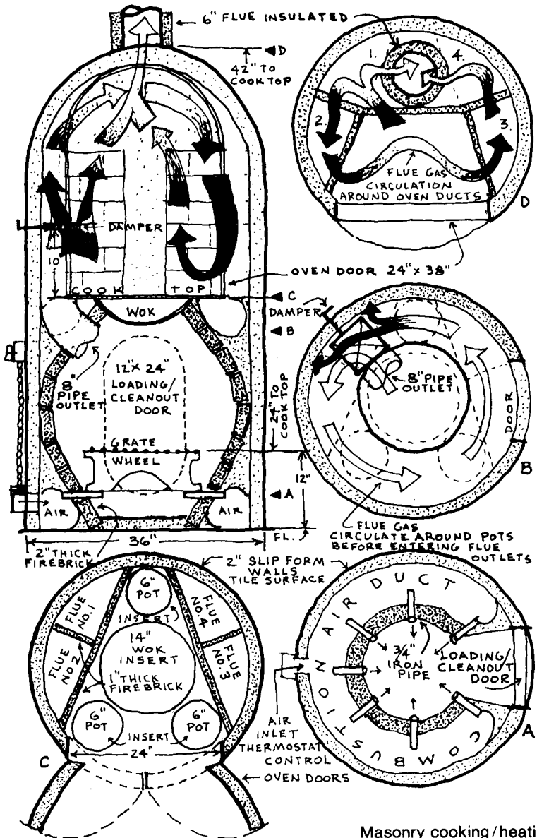
Masonry cooking/heating stove
